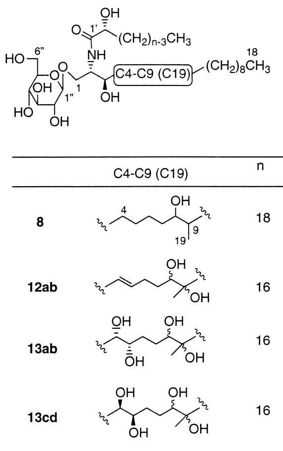
Figure 3. Structures of cerebroside derivatives.
