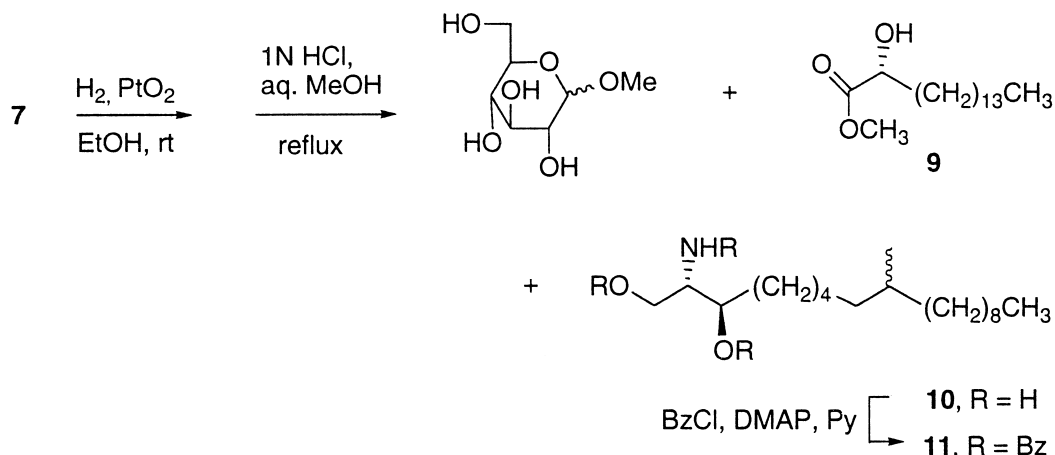
Figure 2. Degradation scheme of 7 .
