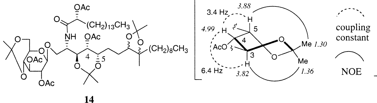
Figure 4. NMR analysis of tetraacetate triacetonide derivative 14 obtained from 13ab to determine the absolute configuration of C4–C5 of 13ab . Partial chemical shifts (in ppm) are in italics .
